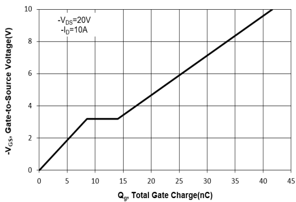
Fig. 11 Gate Charge
