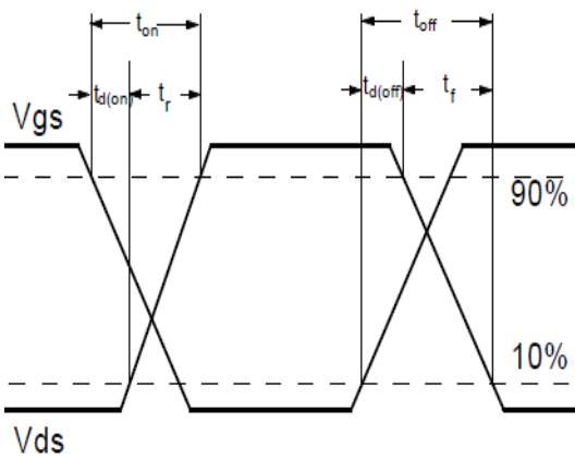
Fig.1-2 Switching Waveform
